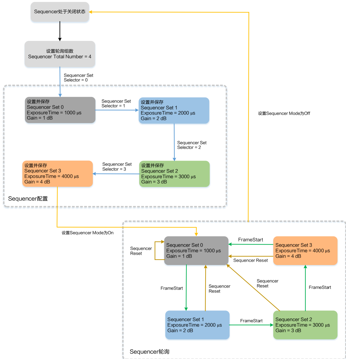
图11-28 Sequencer 轮询
